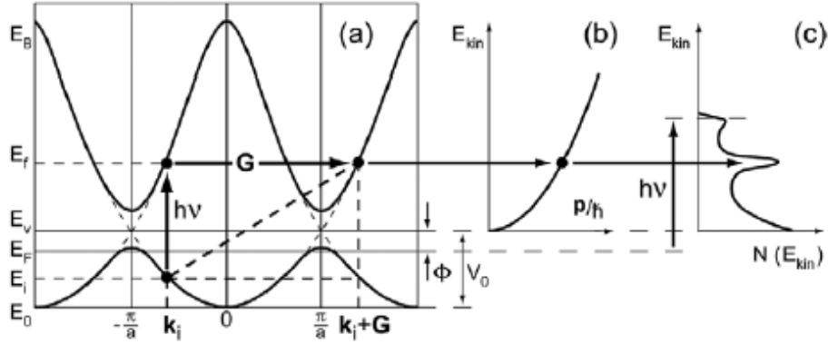
Figure 2.3 Three-step model of a photoemission process. Adapted from [5].
