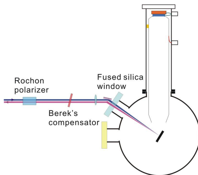
Figure 4.16 Optical diagram to use a Rochon polarizer and Berek compensator to compensate for the window birefringence.
