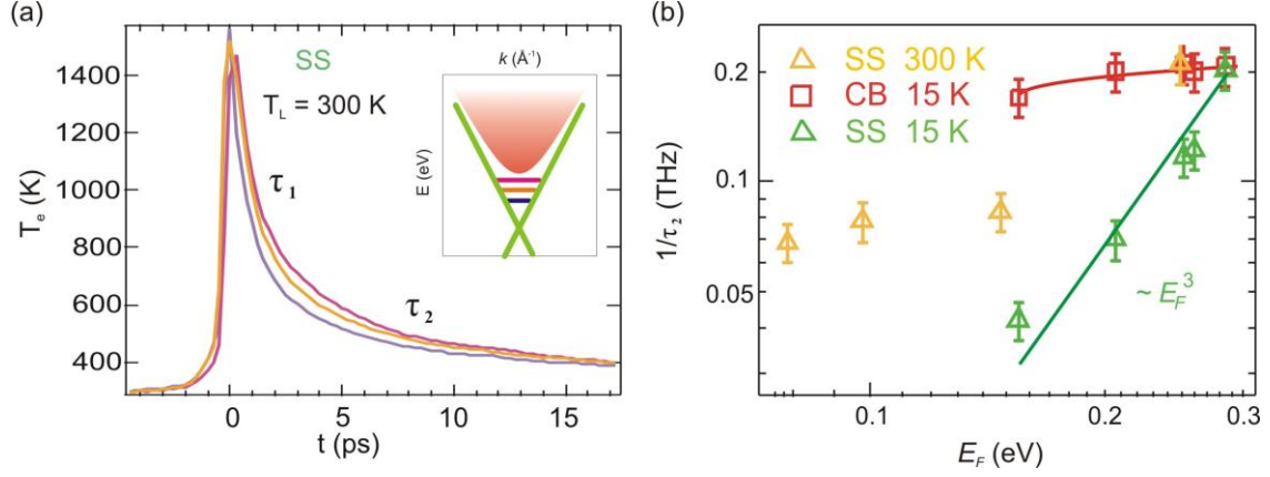
Figure 5.15 Slow component doping dependence. (a) Doping dependence of electronic temperature of SS at 300 K. The color of the trace matches the color of the Fermi level shown in the inset. Both the fast ( \tau_1 ) and slow ( \tau_2 ) components are slightly dependent on the doping. (b) 1/\tau_2 obtained from biexponentially fit the electronic temperature.
